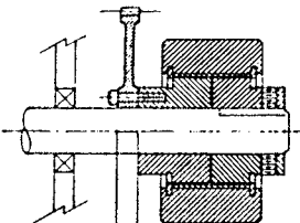
CONCENTRIC SHAFT
