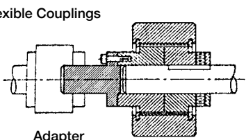
IN-LINE SHAFT
