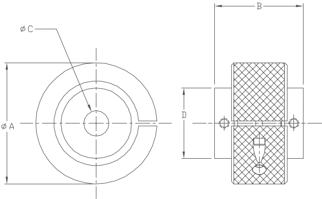
IN-LINE SHAFT
